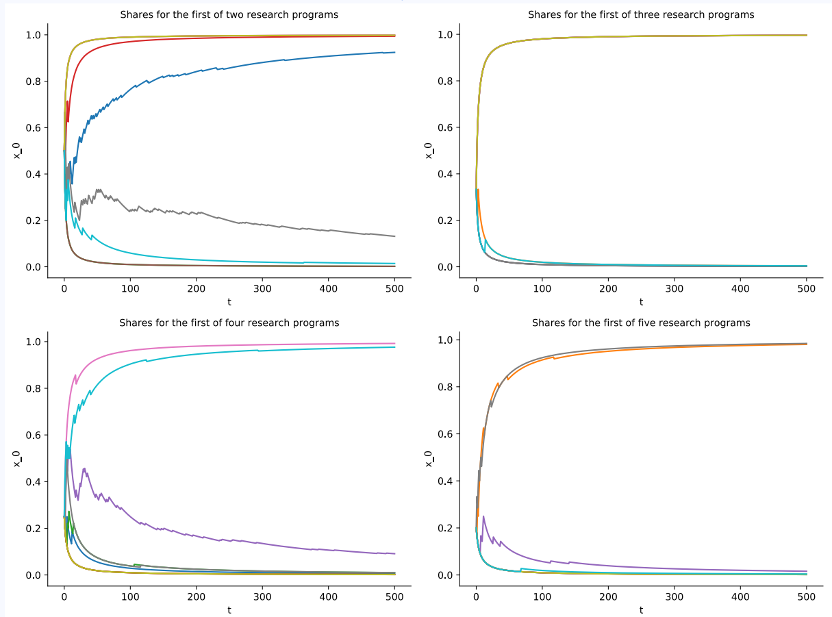
Figure 3: Selected dynamics for the model. In all cases we see that a research program either becomes dominant and takes over large parts of the population, or gets slowly extinct.
